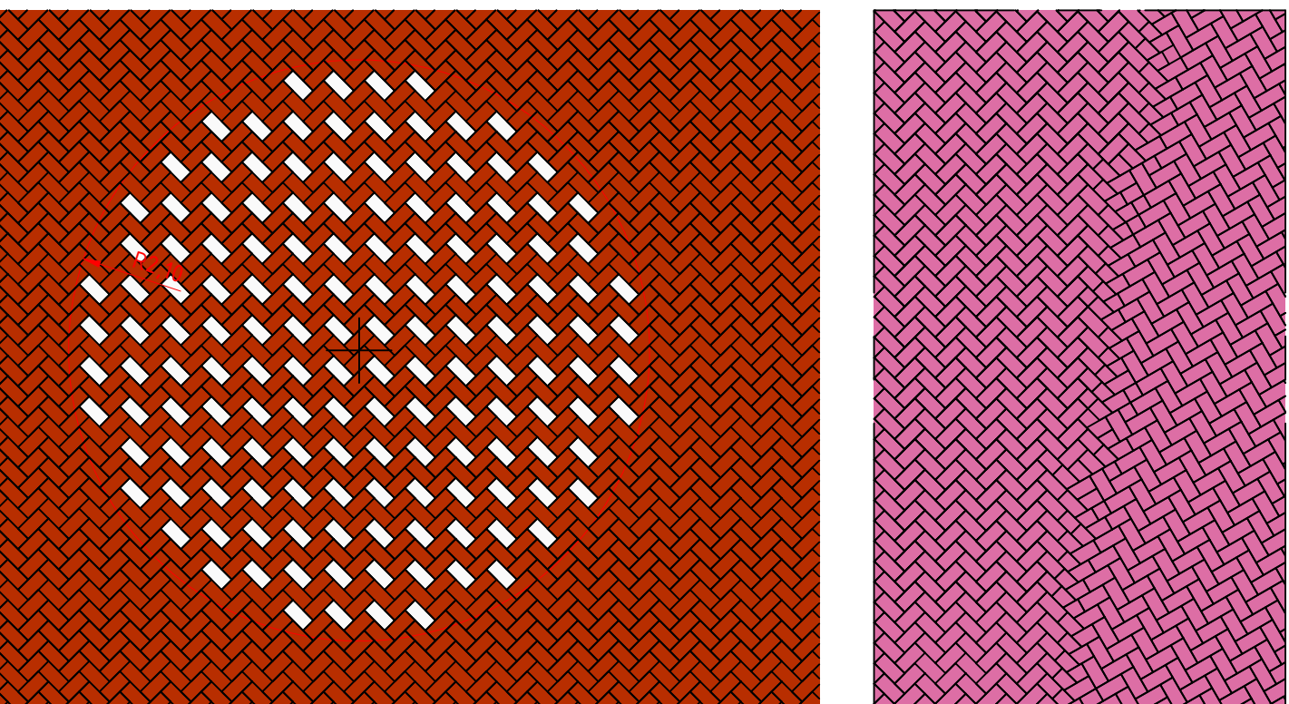
Principedetail markering kruising 1:50
