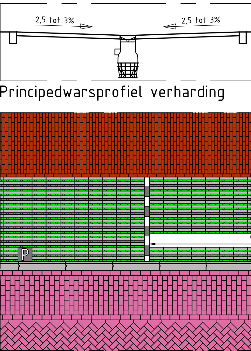
Principedetail langs parkeren 1:50
