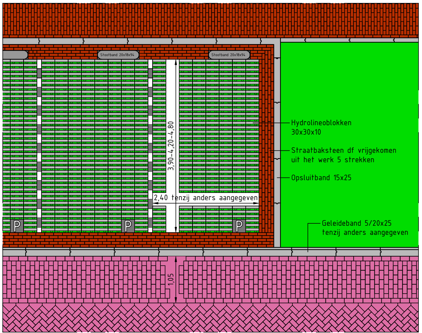
Principedetail haaks parkeren 1:50
